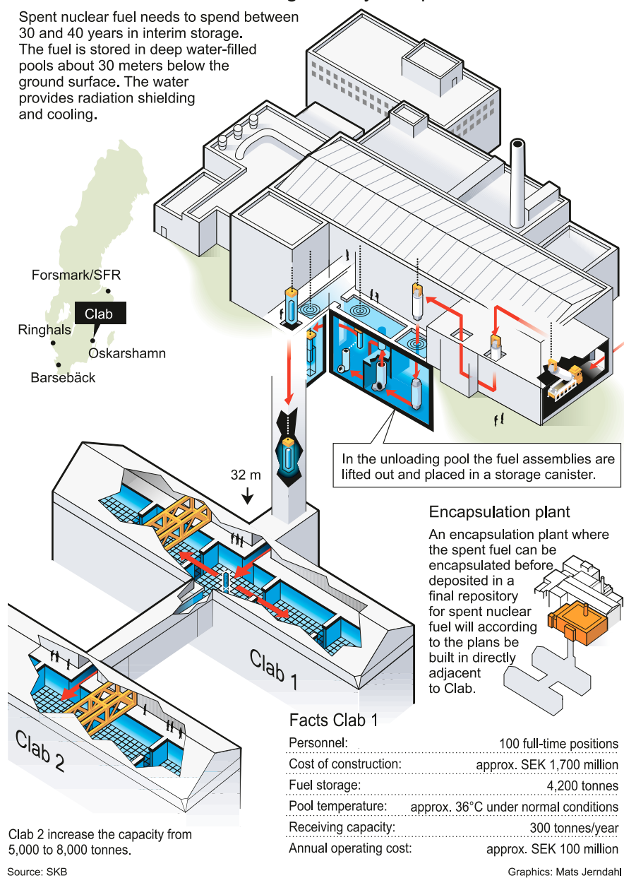
Figure D2: The Clab facility.
