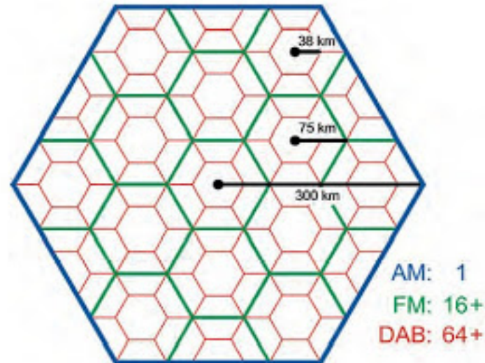
NUMBER OF TRANSMITTERS REQUIRED FOR AM, FM AND DAB BANDS TO COVER A 300 KM RANGE WITH AT LEAST ONE AUDIO CHANNEL
